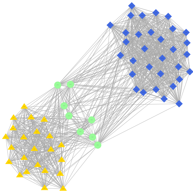
Fig. 10. Applying Kamada-Kawai layout to dataset ‘BT’, a set of nodes in Bordeaux and Toulouse, using the same rendering options as for Figure 9. Toulouse is represented here by diamonds; the ground truth clusters represented by circles and triangles both belong to Bordeaux. Our non-hierarchical clustering method does not recover this ground truth; it finds only two clusters, one for Toulouse and one for Bordeaux. The third ground truth cluster is distinct in the visualization, however, showing that the BitTorrent measurements do reflect it.
