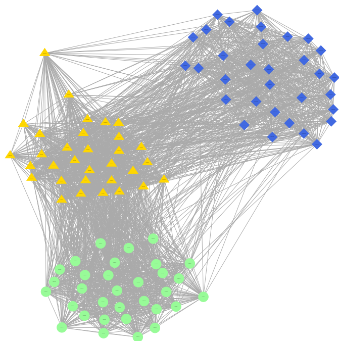
Fig. 12. Applying Kamada-Kawai layout to dataset ‘BGT’, with nodes in Bordeaux, Grenoble and Toulouse, using the same rendering options as for Figure 9.
