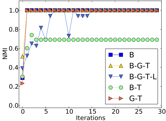
Fig. 6. Comparison of the clustering found using our tomography method, against the ground truth clustering provided. The results are shown in terms of Normalized Mutual Information [32]. We observe that, in general, the NMI improves as the number of measurement iterations performed increases, converging on a stable value. The convergence occurs quickly on the simpler topologies. The NMI frequently converges to 1 – perfect agreement with the ground truth. In the case where NMI does not converge to 1, visualized in Figure 10, we can see that a hierarchical ground truth, and clustering approach, may improve this. Details of the topologies between the four sites used – B ordeaux, G renoble, T oulouse and L yon – are provided in Section IV-A.
