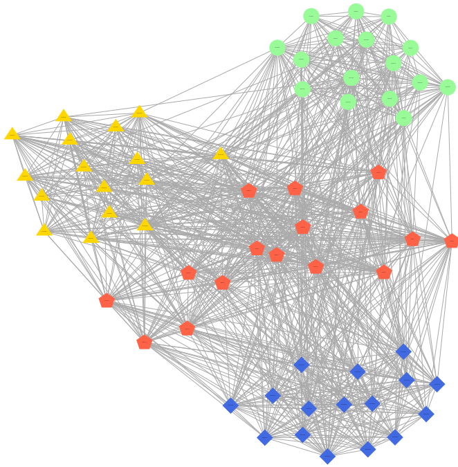
Fig. 13. Applying Kamada-Kawai layout to dataset ‘BGTL’, Bordeaux, Grenoble, Toulouse and Lyon, using the same rendering options as for Figure 9. The ground truth clusters in this rendering appear to be visually less distinctly laid out than the other examples; however, we note that the algorithmic clustering method still achieves perfect accuracy – see Figure 6.
