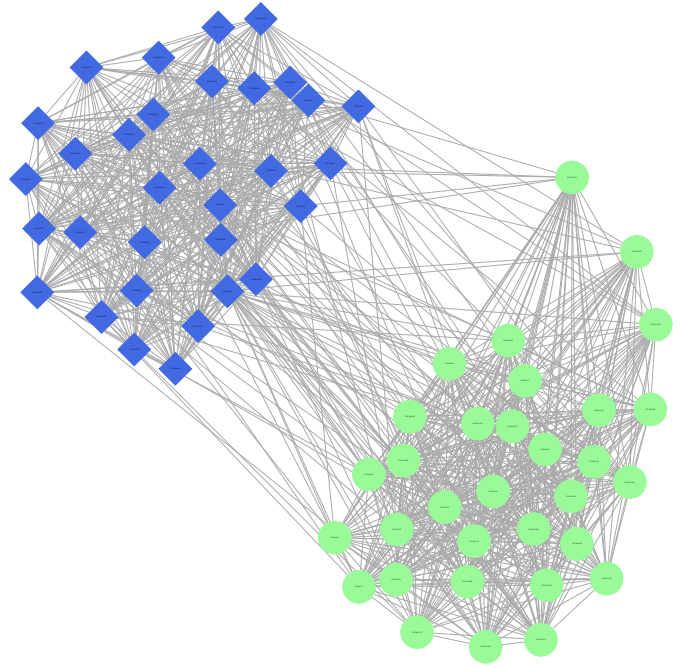
Fig. 9. Applying Kamada-Kawai layout (using the Graphviz’ ‘Neato’ tool) to dataset ‘B’, the Bordeaux site. The configuration used has 64 nodes, divided between 3 physical compute clusters. These 3 physical compute clusters give rise to only 2 logical network clusters, as there is a fast link between the ‘Bordereau’ and ‘Borderline’ physical clusters. The shape and color of each node rendered reflects the labelling of the ground truth cluster it is in. We render only the edges in the top half of all edges, by weight. While the graph is too dense to visually make out any structure due to edge weight, it is clear that the layout algorithm is grouping nodes corresponding to their ground truth. This provides grounds for expecting a graph clustering algorithm to find these clusters.
