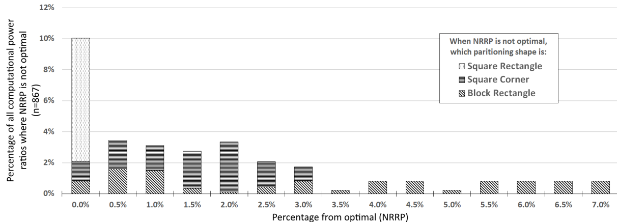
Figure 12: Percentage from optimal for all computational power ratios where NRRP is not optimal, and which partition shape is optimal in these cases.
