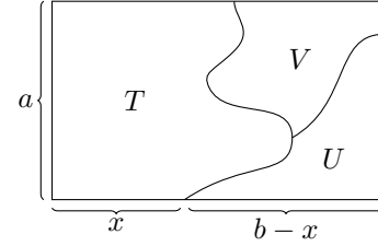
Figure 4: Notation for the case where one processor holds a complete side
