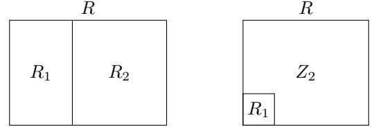
Figure 6: An illustration of the Guillotine (left) and Square (right) routines.
