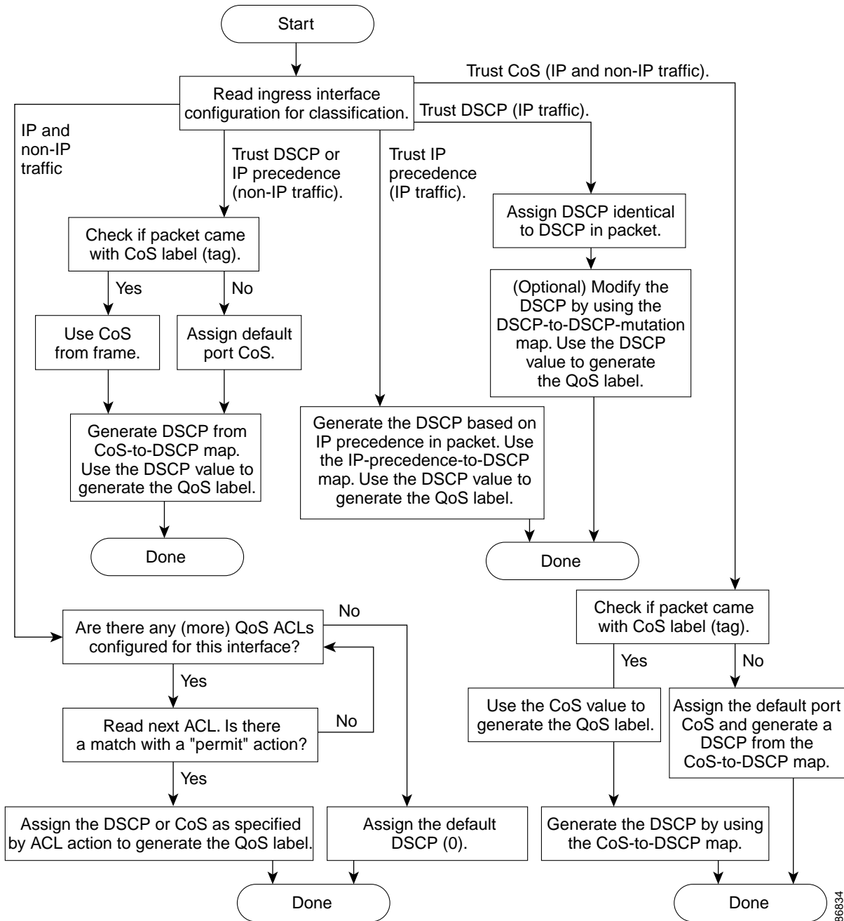
Figure 31-3 Classification Flowchart
