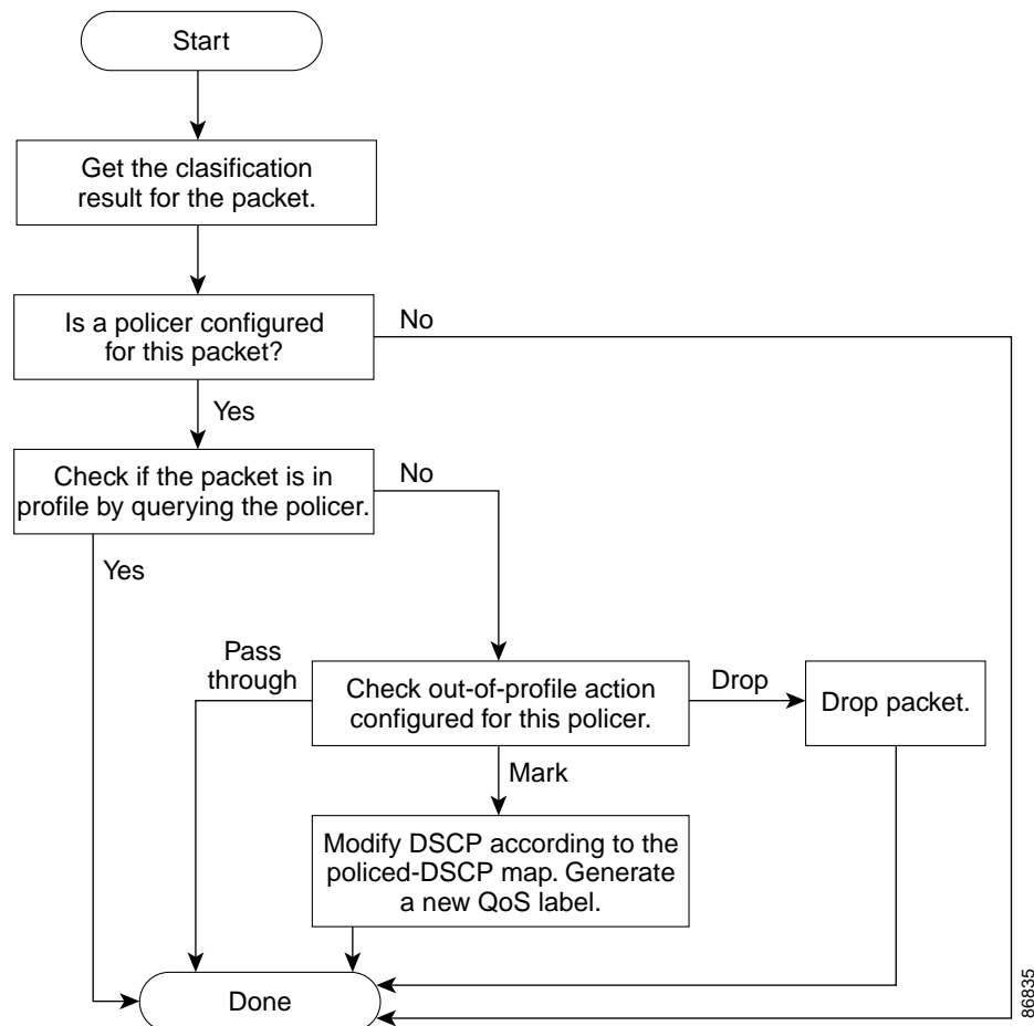
Figure 31-4 Policing and Marking Flowchart
