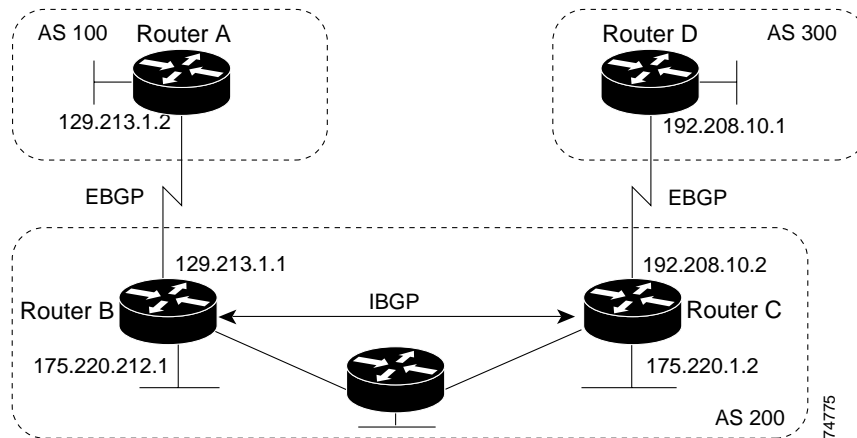
Figure 33-4 EBGP, IBGP, and Multiple Autonomous Systems
