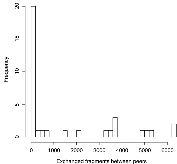
Fig. 5. Distribution of measured metric w(e) for a fixed edge e and 36 independent iterations.
